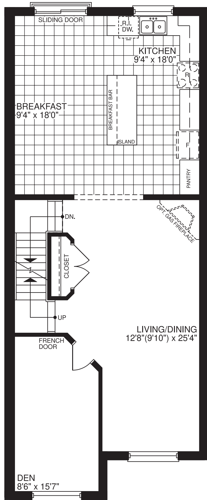
MAIN LEVEL ELEVATION A & A1
