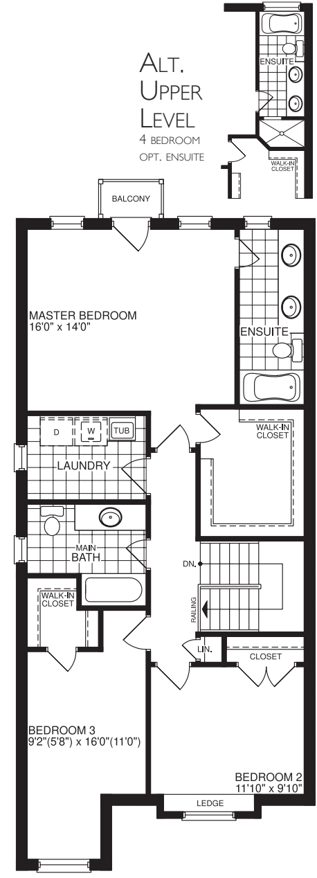
ALT. UPPER LEVEL 4 BEDROOM
